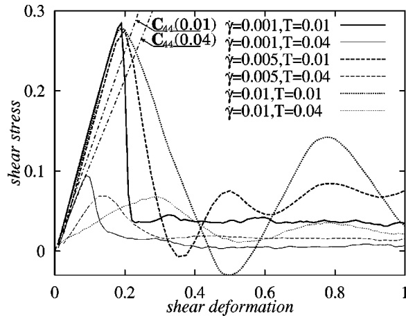
FIG. 5. Shear stress as function of deformation for three shear rates \dot{\gamma}=0.001, 0.005 , and 0.01 at two temperatures T=0.01 (thicker curve) and T=0.04 (thinner curve) of GEAM, obtained via NEMD. The starting configuration is the ideal fcc structure at density n=1.00 with N=43\,000 particles. The shear started at t=0 . Shear direction is the [100] direction in crystal, and shear plane coincides with the (010) crystal plane. The coefficient C_{44} is obtained via MD simulation. All quantities are given in LJ units.
