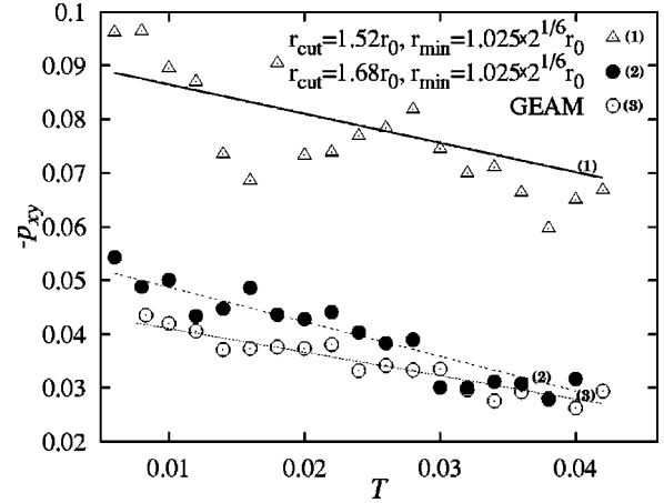
FIG. 7. Shear stress as function of temperature (in standard LJ units) for different model parameters, minimum r_{min} and cutoff radius of the potential r_{cut} . Symbols denote averages from the NEMD simulation at shear rates \dot{\gamma} = 0.001 . Curves are obtained by linear regression analysis of the simulation results.
